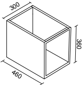
Base a giorno Open base cabinet
