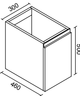
Base sospesa con 1 anta Wall cabinet with 1 door
