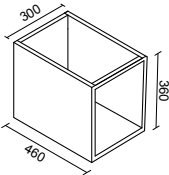
Base a giorno Open base cabinet
